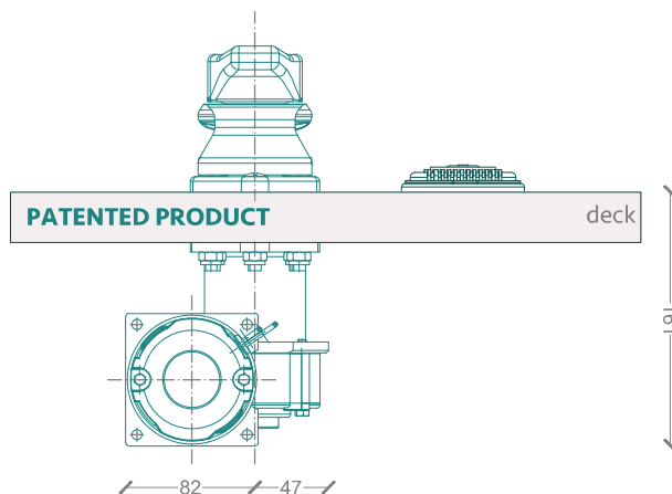
TRASVERSAL SECTION
