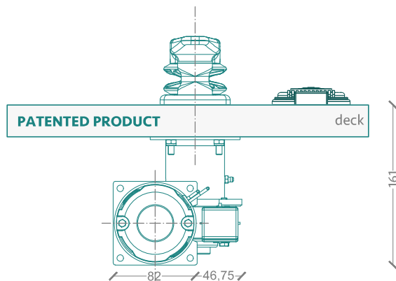
TRASVERSAL SECTION
