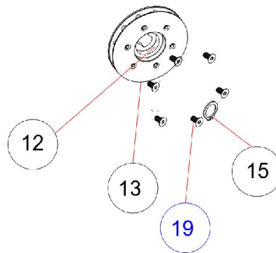
A3SP04001 - Sprocket - 1543-SP.Z12 QTH
